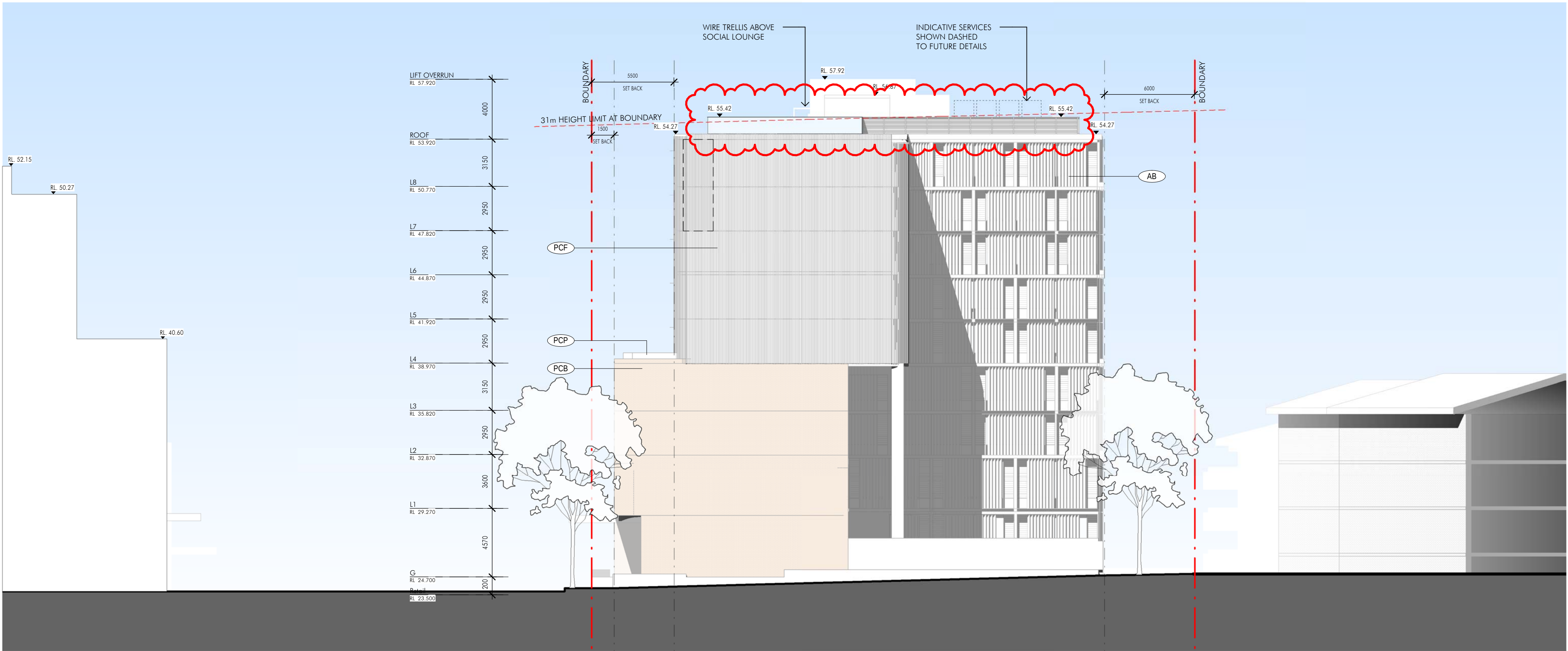
2 Elevation - North West - Proposed 1 : 200
