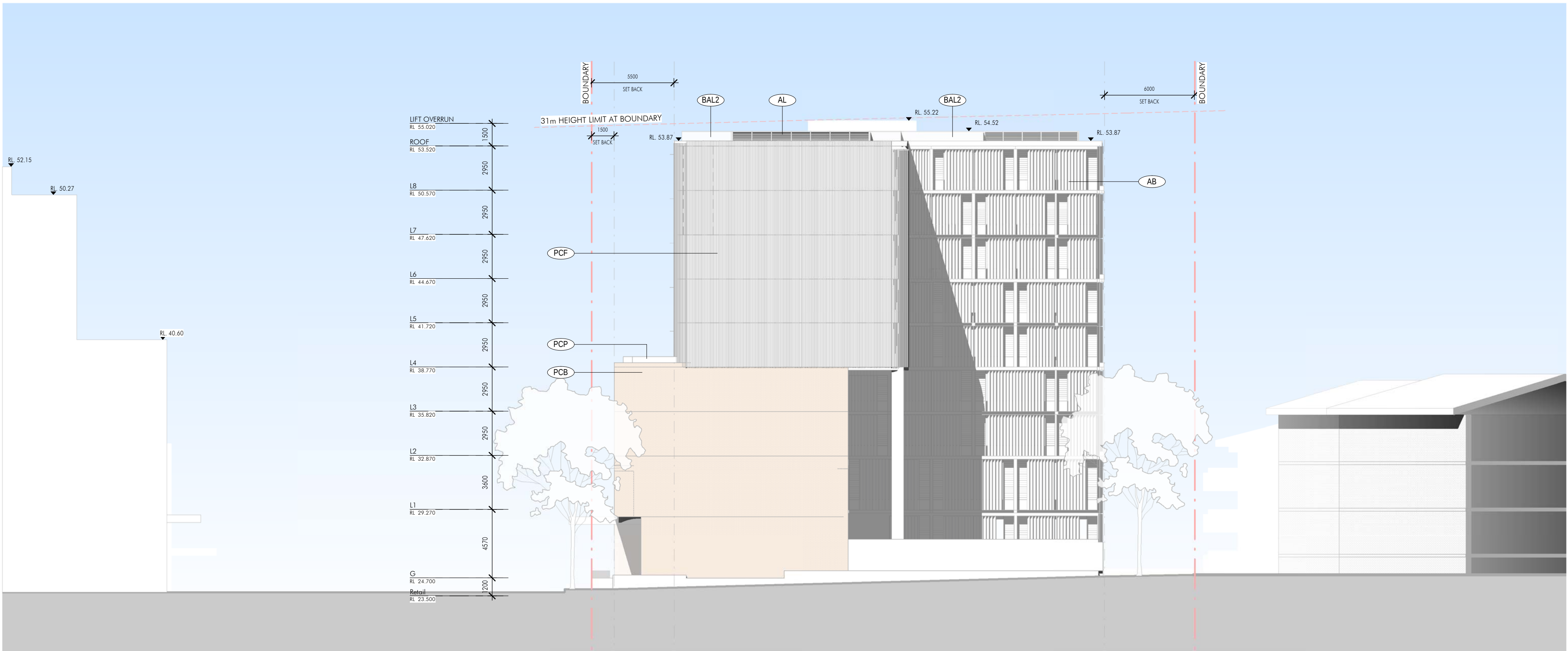
1 Elevation - North West - Approved 1 : 200
